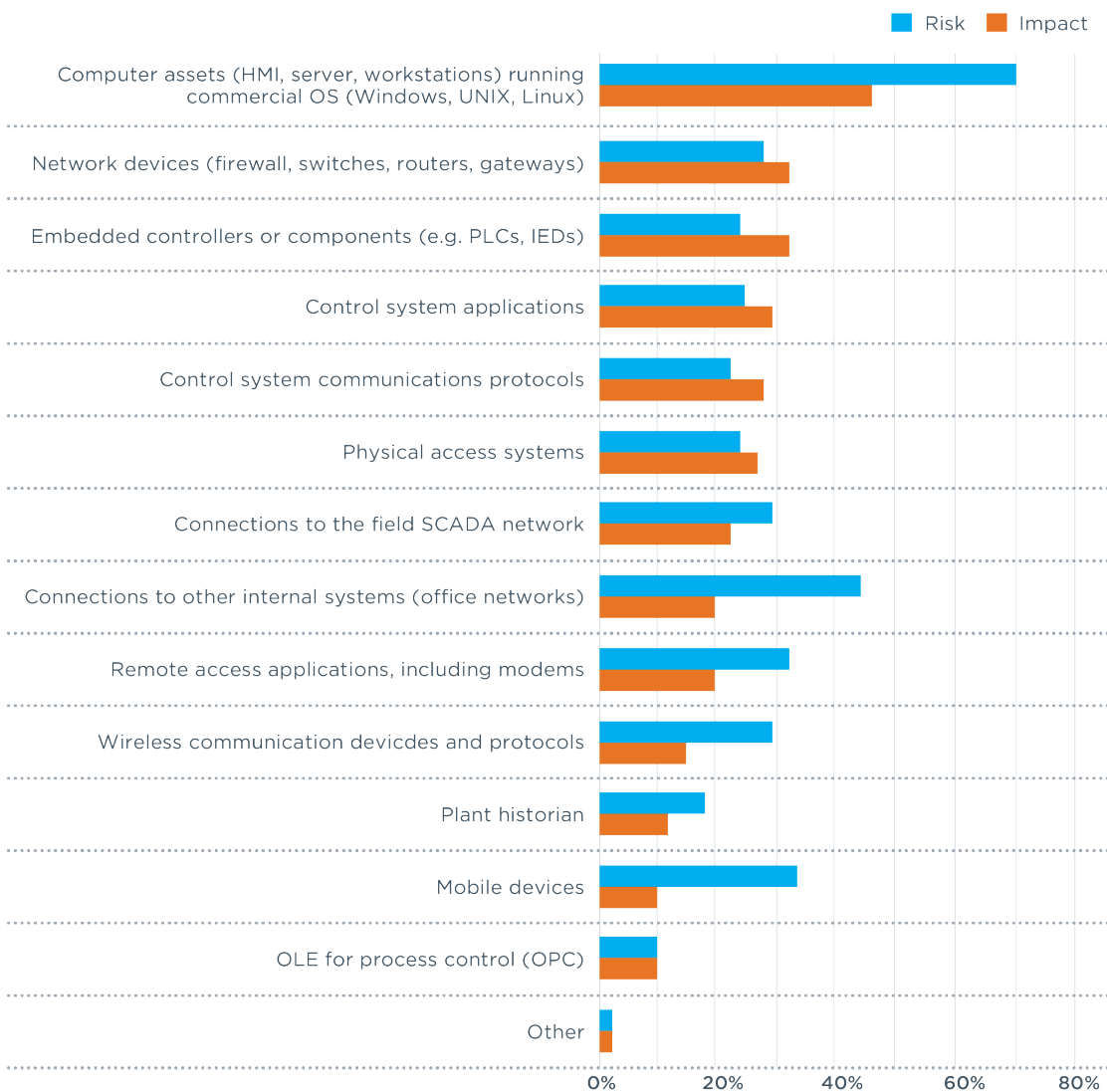
Figure 4: Network components that are most at risk (Source: SANS Securing Industrial Control Systems-2017 survey) 32
