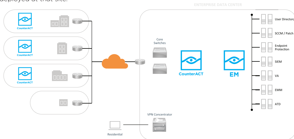
Figure 6: ForeScout hybrid deployment
