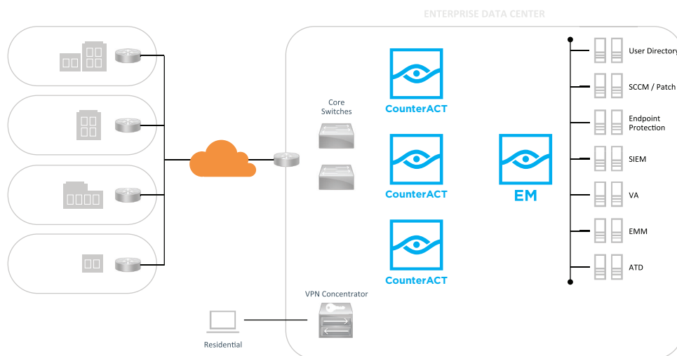
Figure 4: ForeScout centralized deployment
