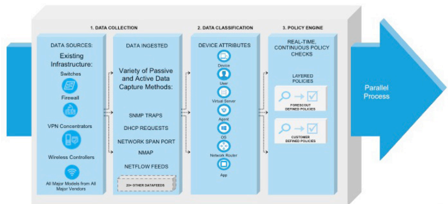
Figure 2. ForeScout uses passive techniques to discover, monitor and assess devices
